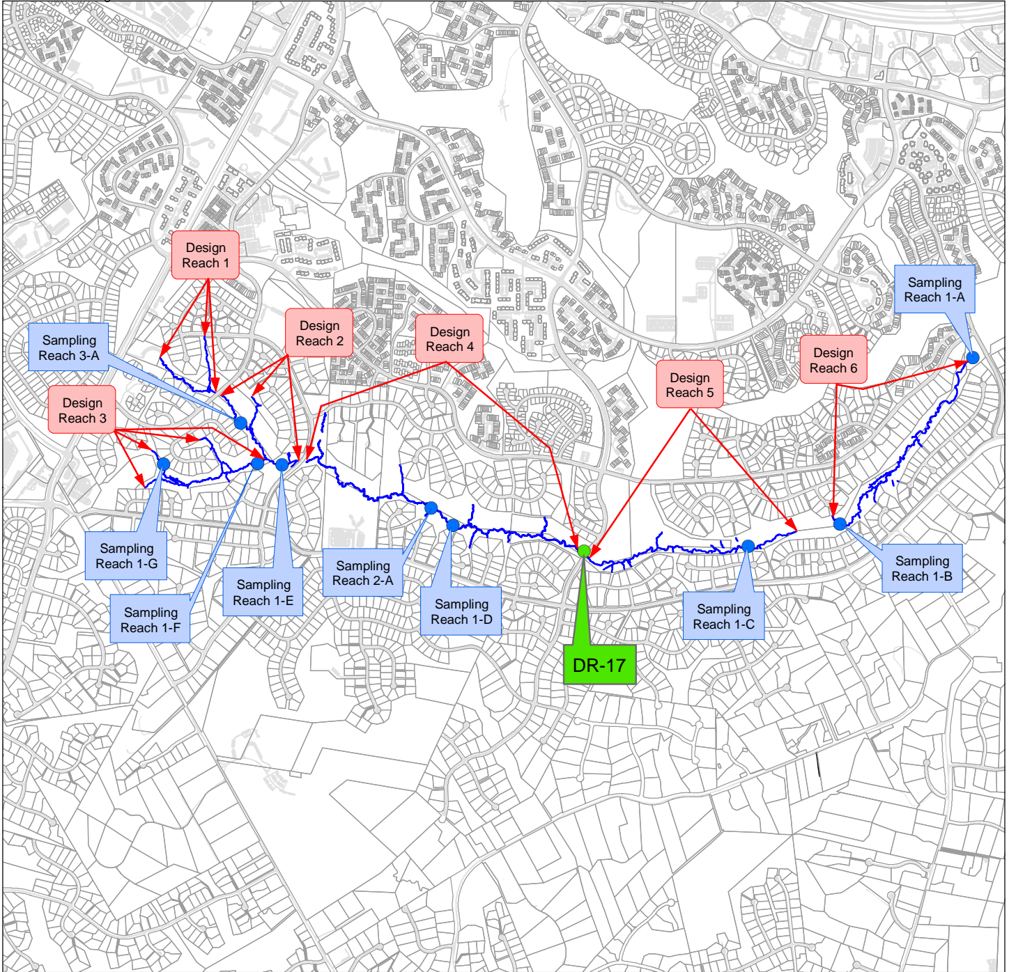
Restoration Design and Sampling Reach Location Map The Glade WSSI #20030 Scale: 1" = 2000'
